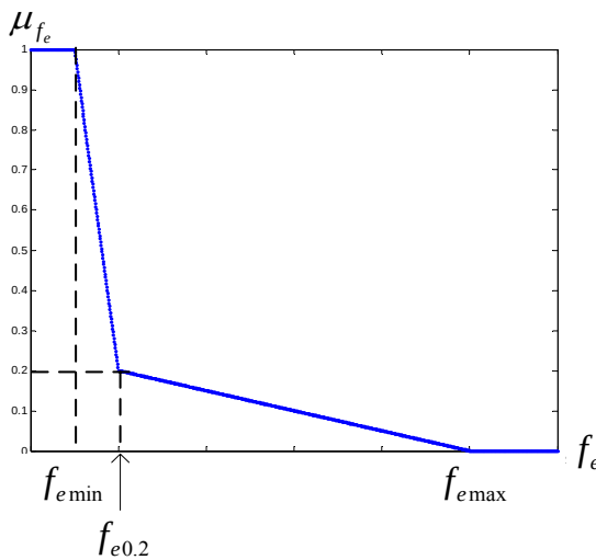
Fig. 2. Fuzzy membership function of the power loss
