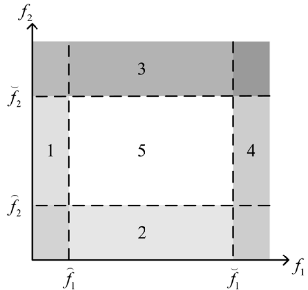
Fig. 7. Decision region on a two-objective space.
