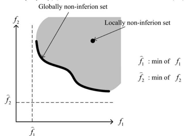
Fig.6. Global non-inferior solutions of two-objective optimization problem.
