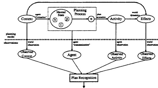
Figure 1: Plan recognition framework.
