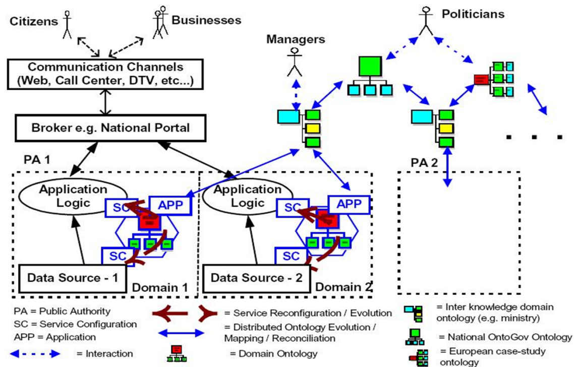
Fig. 3. OntoGov service provision model
